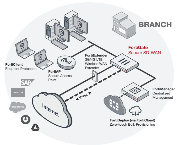
FortiGate 600E deployment in branch office (Secure SD-WAN)
